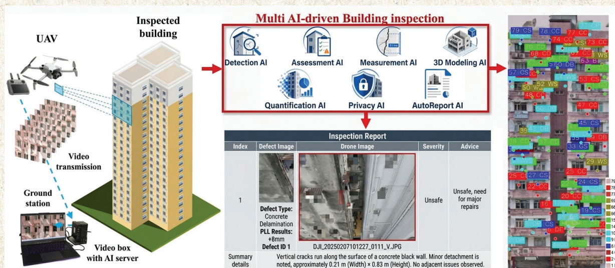
The system links autonomous data capture with defect detection, measurement, assessment, 3D modelling, privacy protection and automated reporting.
